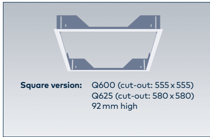
PLASTERBOARD
